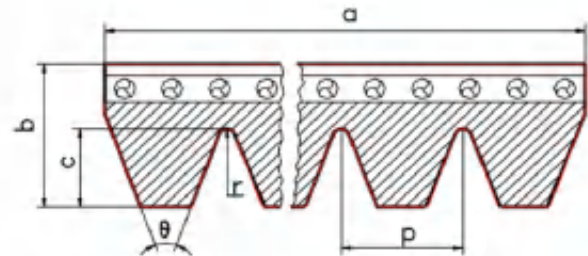
单面槽截面尺寸 SINGLE SIDE SECTION DIMENSIONS
